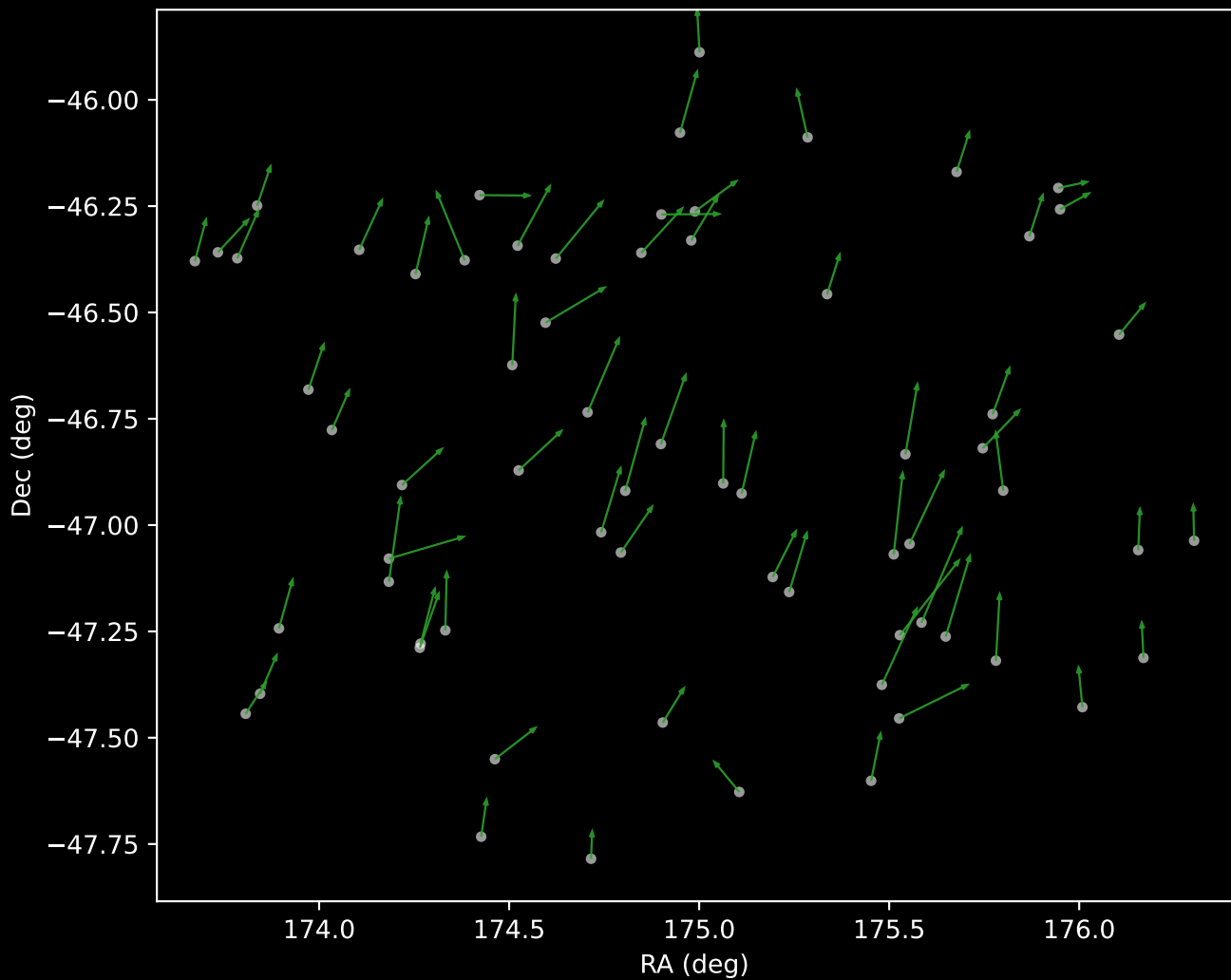
GALAH DR4 Cluster 4 Proper Motion Vectors (n=68)
