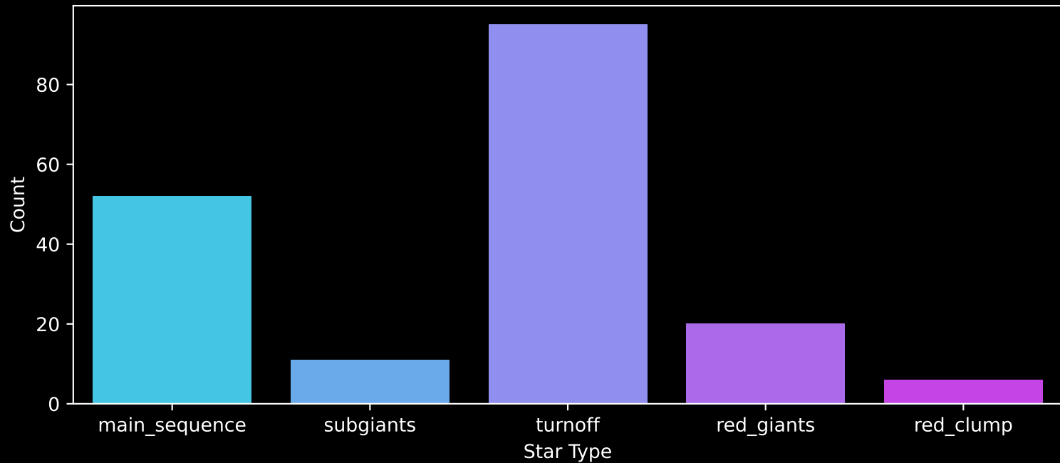
GALAH DR4 Field: [343] Count plot of Star Type
