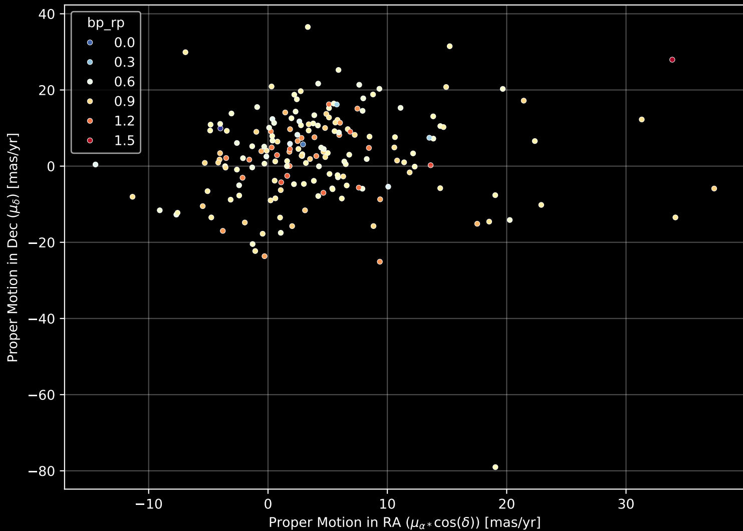
GALAH DR4 Field: [343] Proper Motion Diagram (n= 184)
