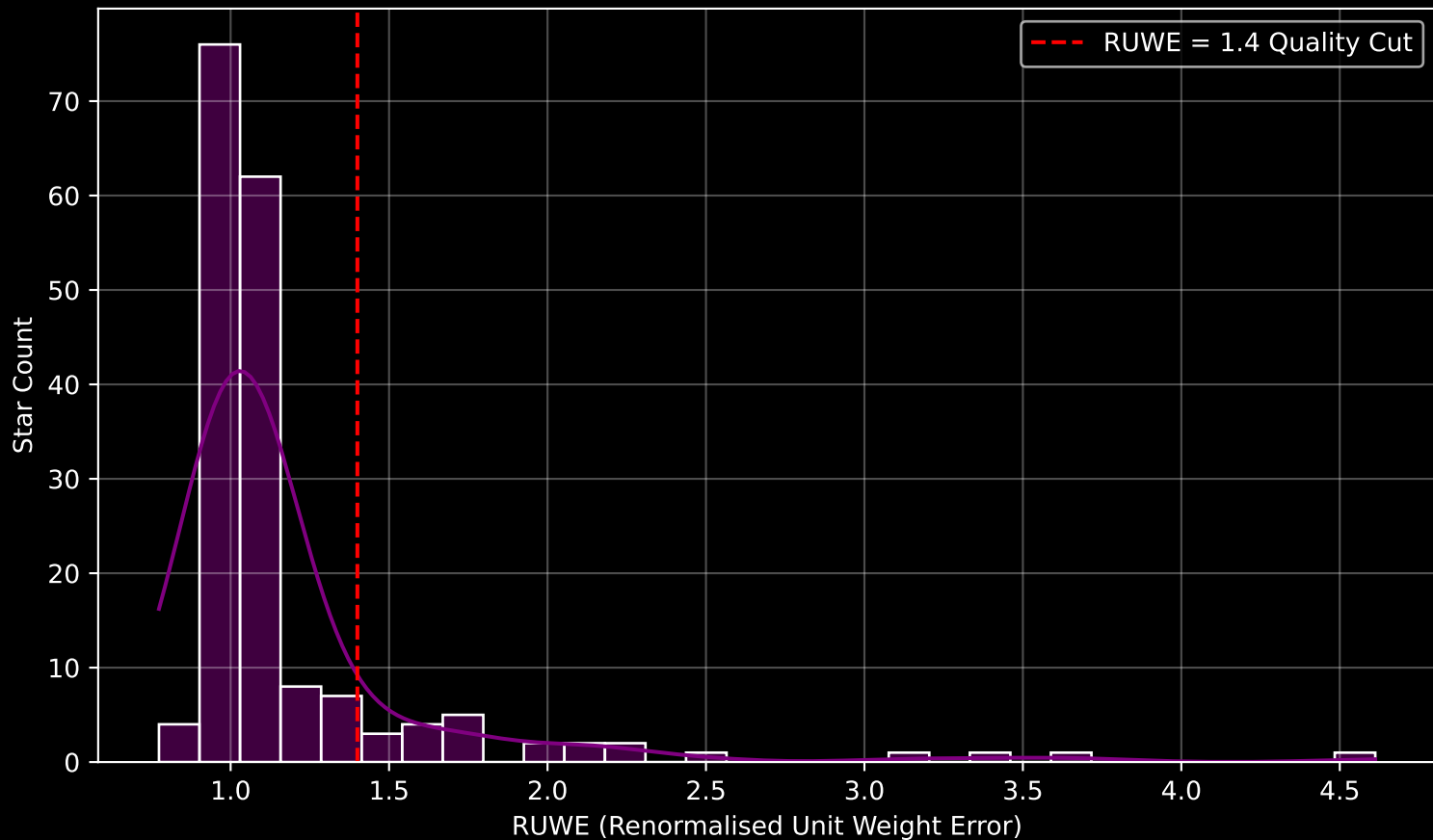
GALAH DR4 Field [343] RUWE Distribution (n= 180)
